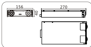
Mechanical Drawing
