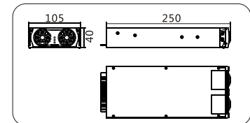
Mechanical Drawing
